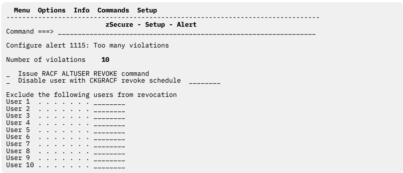
Figure 24. Setup Alert panel: Configuring revocation for excessive violations
